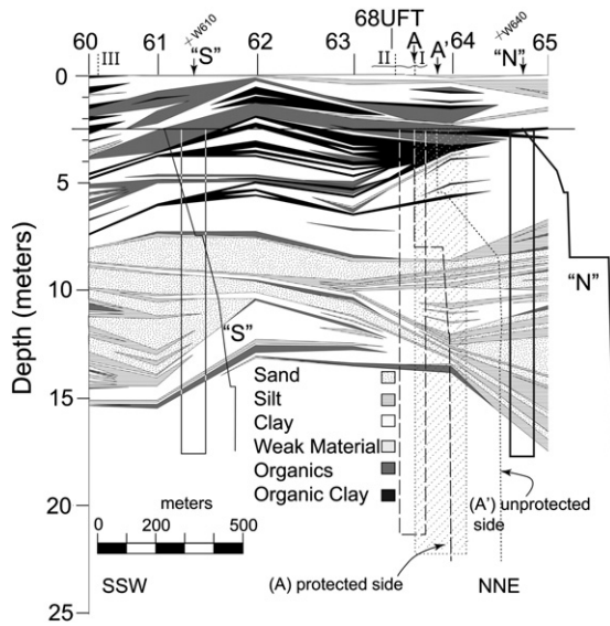
Fig. 11. Integrated CPT and seismic results. Cone-penetrometer test (FFEB, 2007) data-derived cross-section, showing six different interpreted soil behavior types. Four areas enclosed by rectangles show the lateral extent of subsurface sampled by pseudowalkaway profiles projected on to the line, from up to 30 m away, from the east (site A') or west (sites "S", A, "N"). The largest enclosed rectangle corresponds to the pseudowalkaway profile taken on the flood-unprotected side of the levee crest (east). Reference toe-of-levee lies ~2.5 m below the crest. Tests along the center of the artificial levee crest are located at regular intervals, referenced by numbers. Samples for laboratory testing (Figure 4) are taken at well (68UFT), marked with a continuous vertical line. V_S -depth models (Figure 8) are superimposed. Several features shown in Fig. 2 are cross-referenced along the top axis, such as (1) the map shape of the levee crack. (2) Vertical dashed lines locate where topographic profiles cross the levee axis. (3) Crosses locate local levee survey markers (W 610–southernmost, W640–northernmost) along the protected levee flank. (4) Roman numerals locate levee topographic profiles (Figure 5). Depths are referenced to crest of levee elevation, but long horizontal line marks the toe-of-levee elevation.
