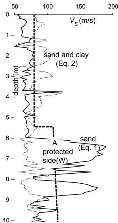
Fig. 12. Applied statistical correlation equations. Two common empirical relations between V_S and CPT data (Hegazy and Mayne, 1995) are applied to tip resistance and sleeve friction values from CPT site 63 (Figures 2, 5, 11). One relation is derived for mixtures of clay and sand (smallest dashes) and another for dominantly, sand (continuous line).
